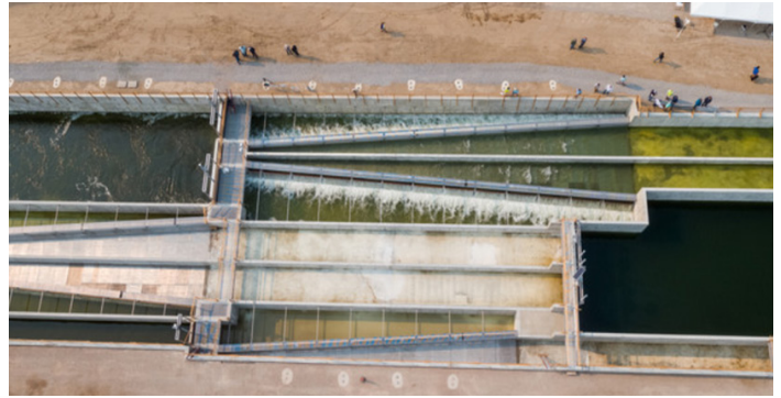
Aerial view of the Derby Dam fish screen.
